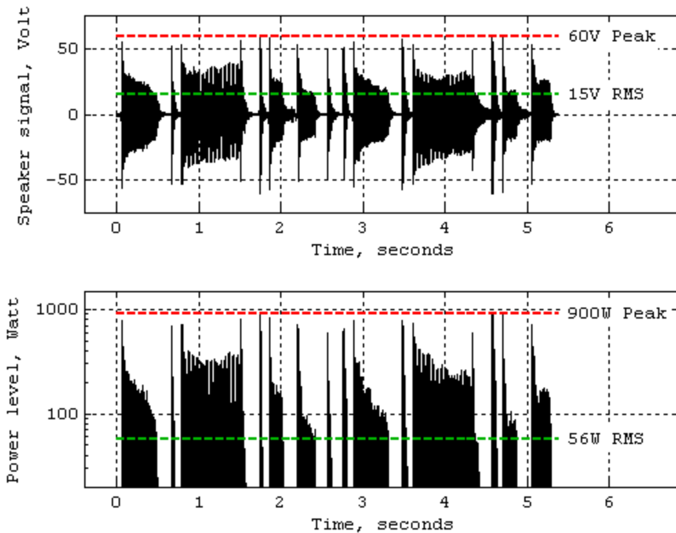
Figure 3: Transistor: Actual vs. Perceived power, crest factor 12dB
