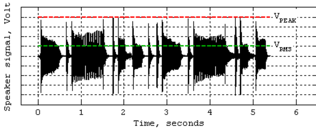
Figure 2: Bass signal with approximated RMS marking / perceived loudness, 12dB crest factor
