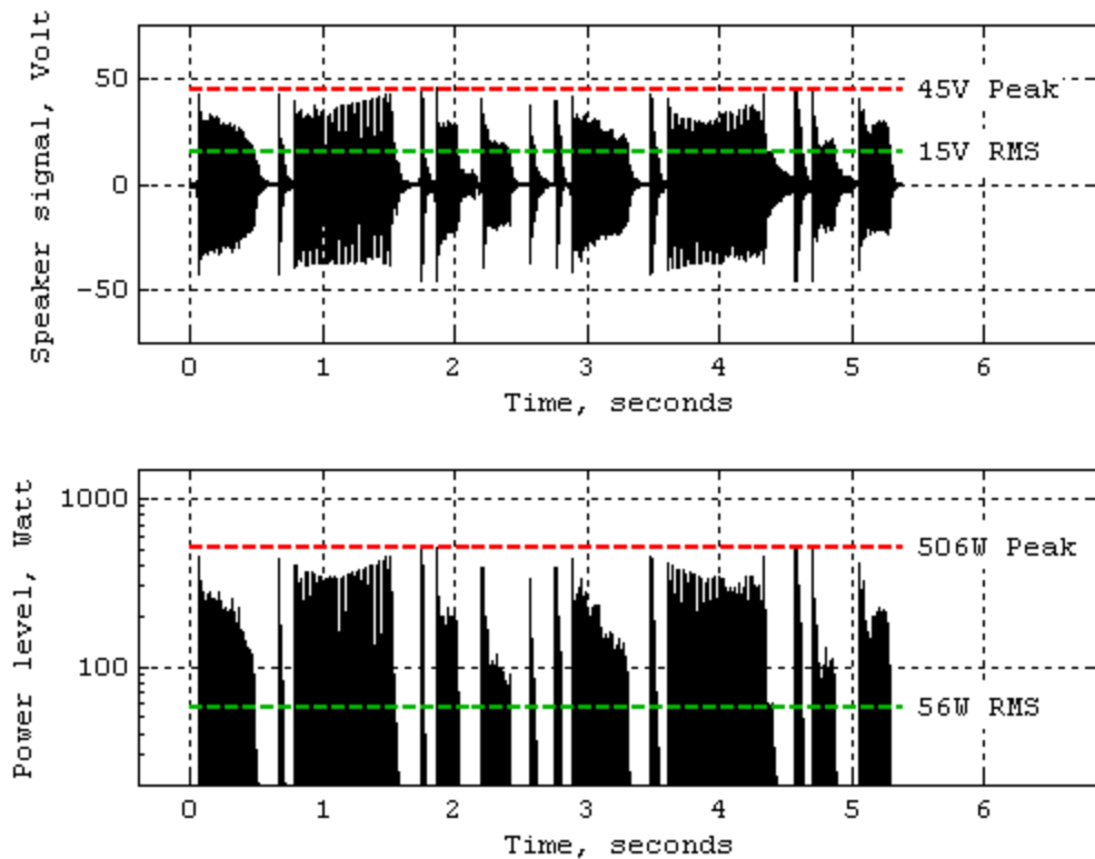
Figure 4: Tube amp: Actual vs. Perceived power
